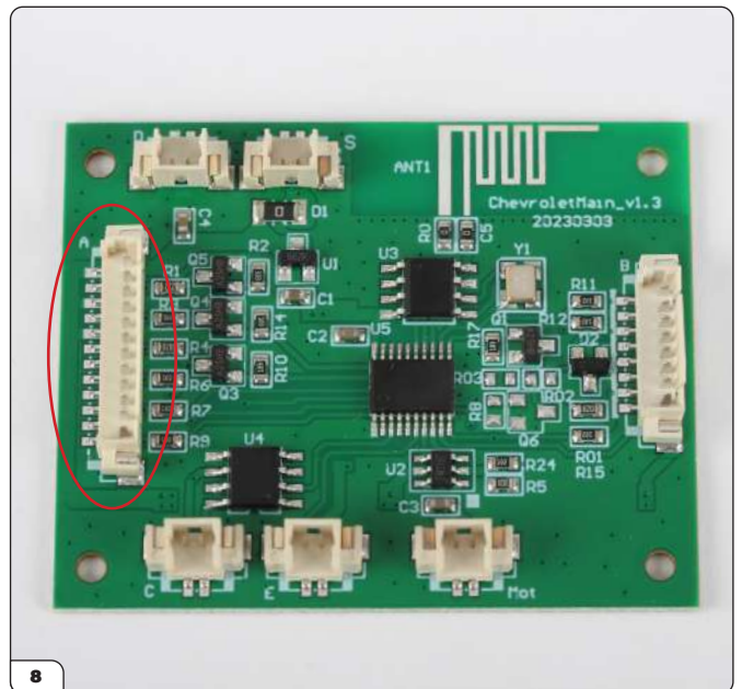
Take the circuit board – each socket is marked with the corresponding cable letter. Note the 'A' socket (circled).
