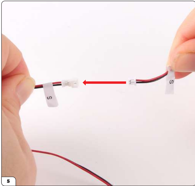
Connect the power switch and the extension cable (both labelled 'S') together as shown.
