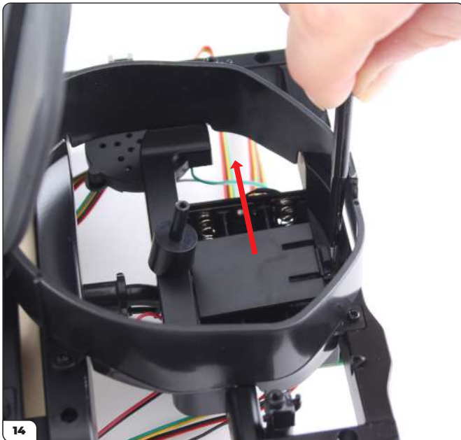
Use tweezers to apply pressure to the clip and remove the battery compartment cover.
